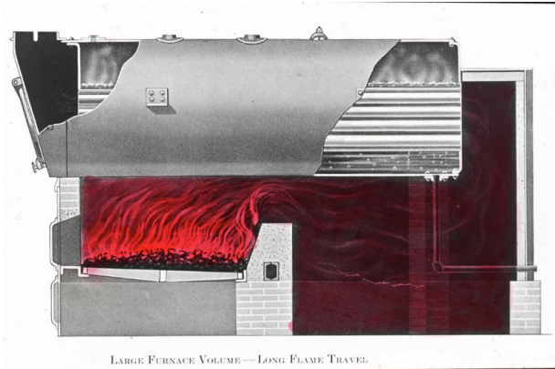
LARGE FURNACE VOLUME — LONG FLAME TRAVEL
