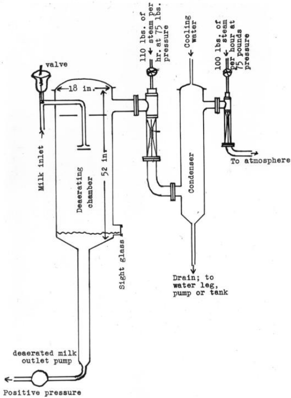
Diagrammatic illustration of continuous milk deaerating unit rated over 3,000 pounds per hour as designed by
